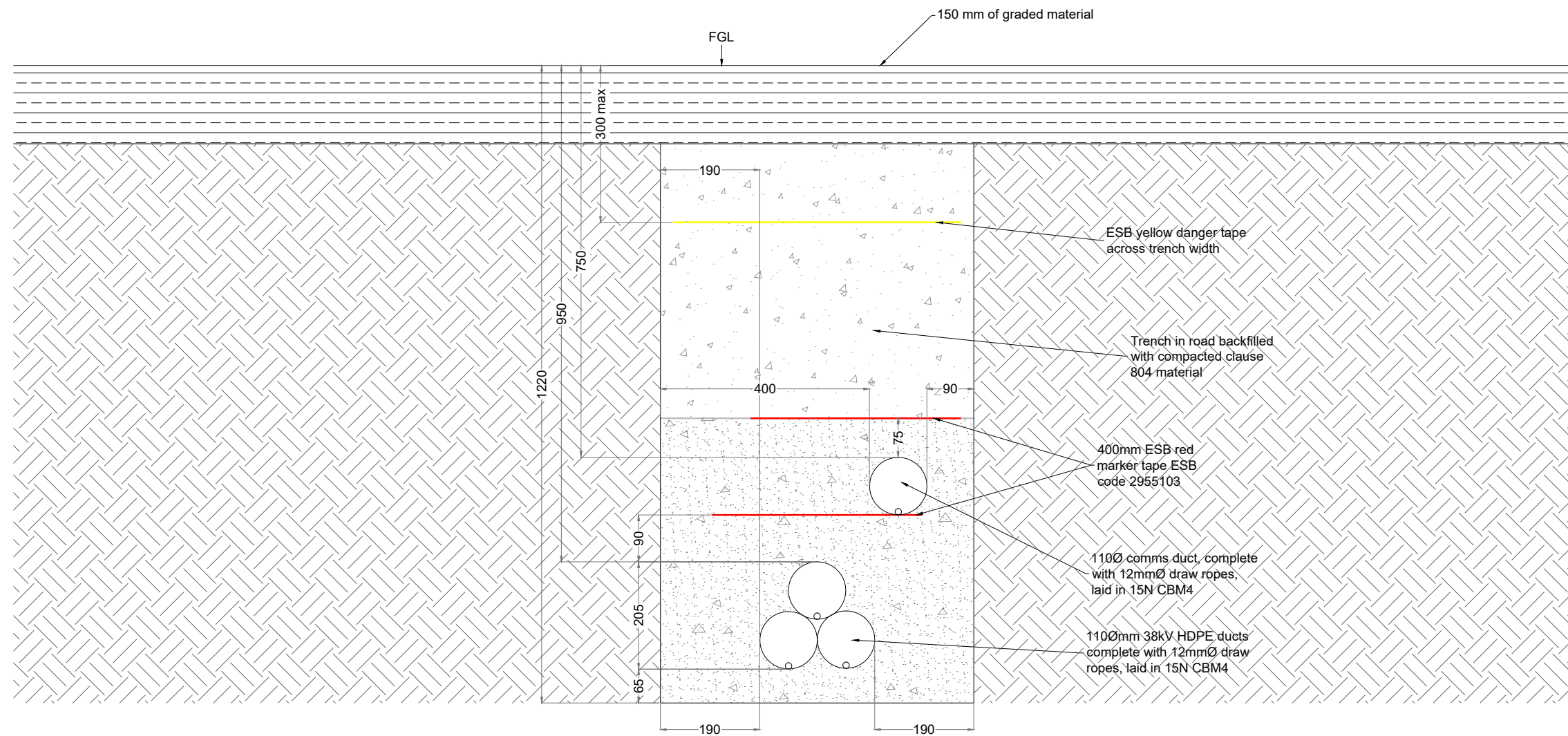
Trench Layout Single Circuit (4-way) Trefoil
