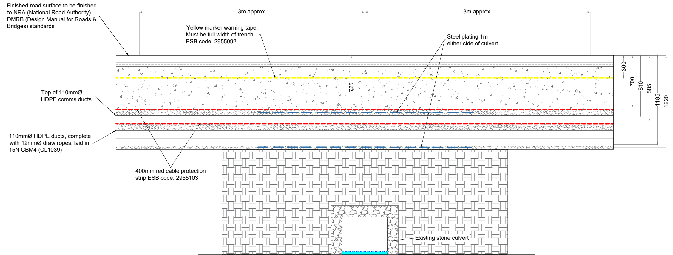
Longitudinal section at watercourse crossing
